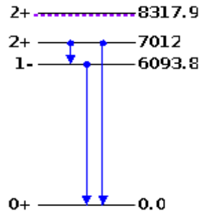
Figure 3: 14C Energy spectrum (KeV)
